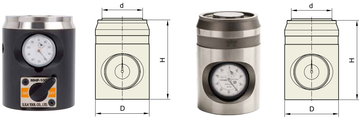
• MAGNETIC HEIGHT PRESETTER
